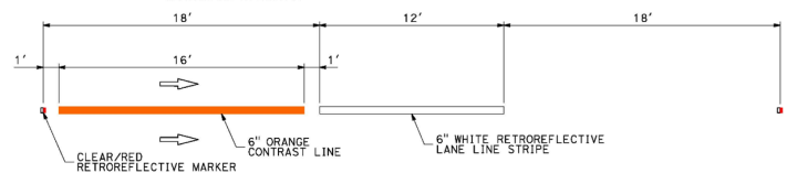
“Orange Preceding White” Southbound Orange Lane Striping Alternative
