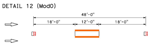
“Orange Along Both Sides” Northbound Orange Lane Striping Alternative
