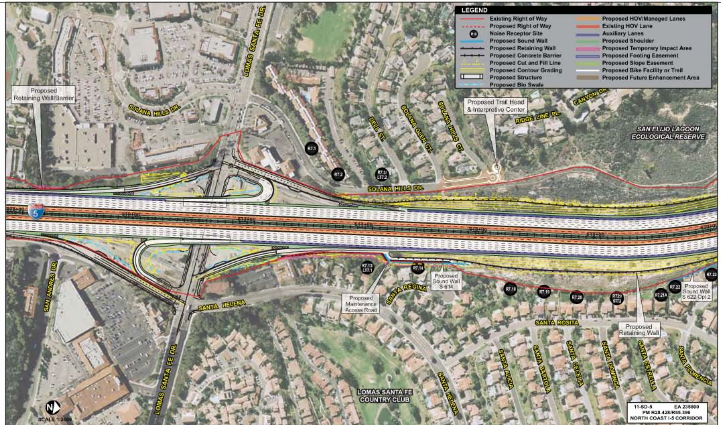
Figure 2-2.14o Project Features Map: 10+4 Buffer Alternative
