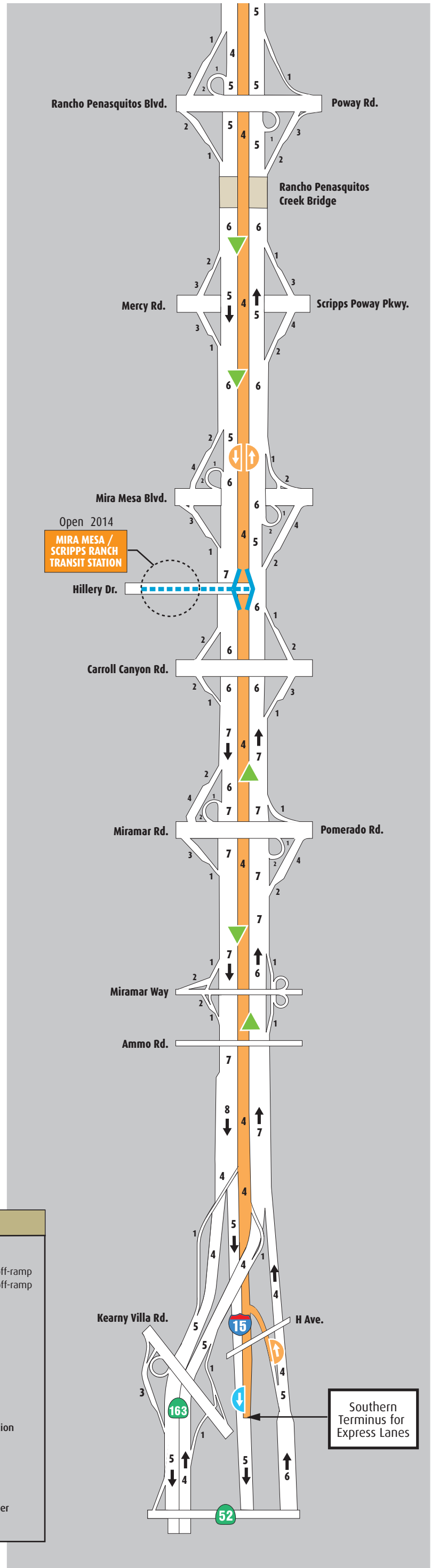
Proposed Lane Configuration Improvements
