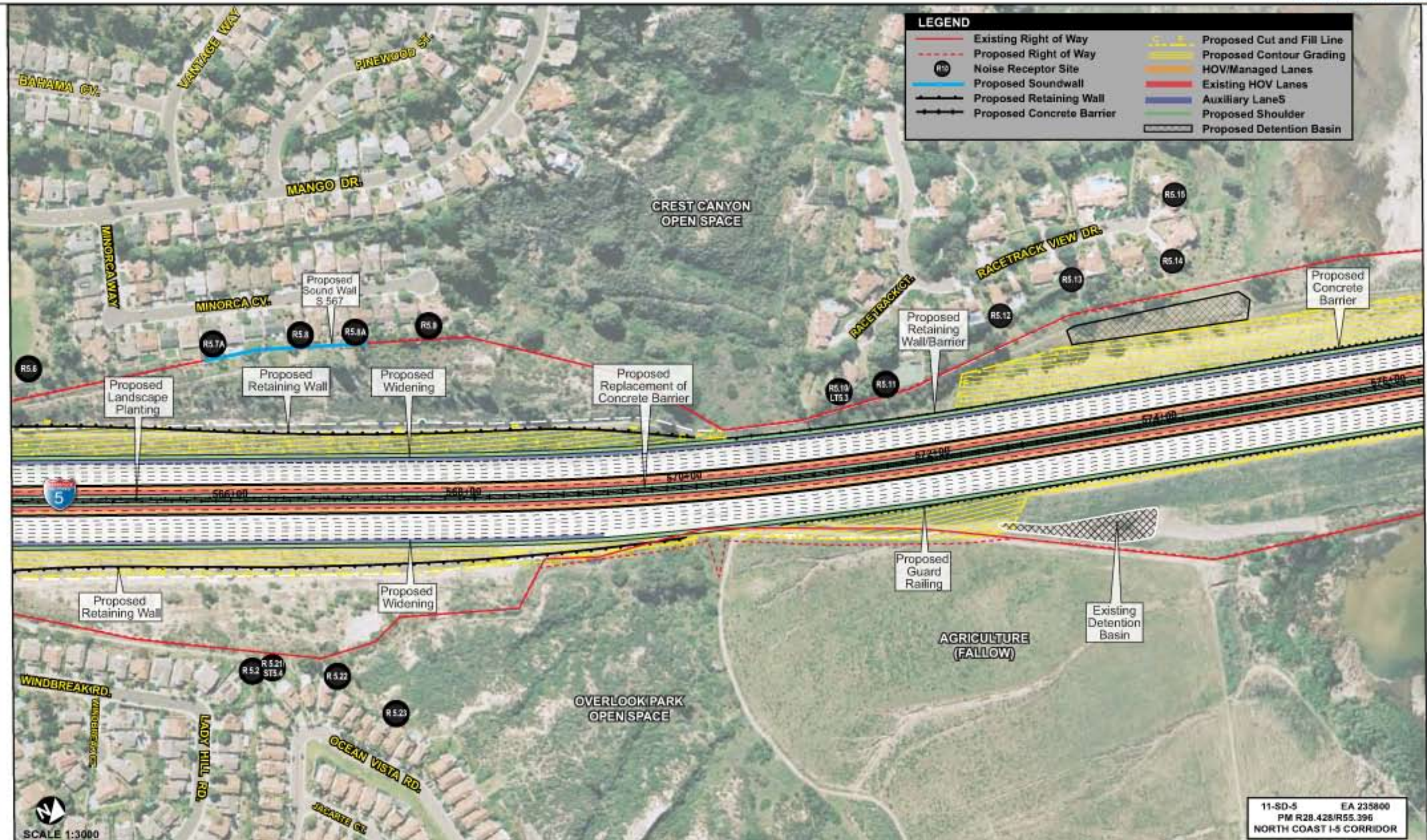
Figure 2-2.14k Project Features Map: 10+4 Buffer Alternative
