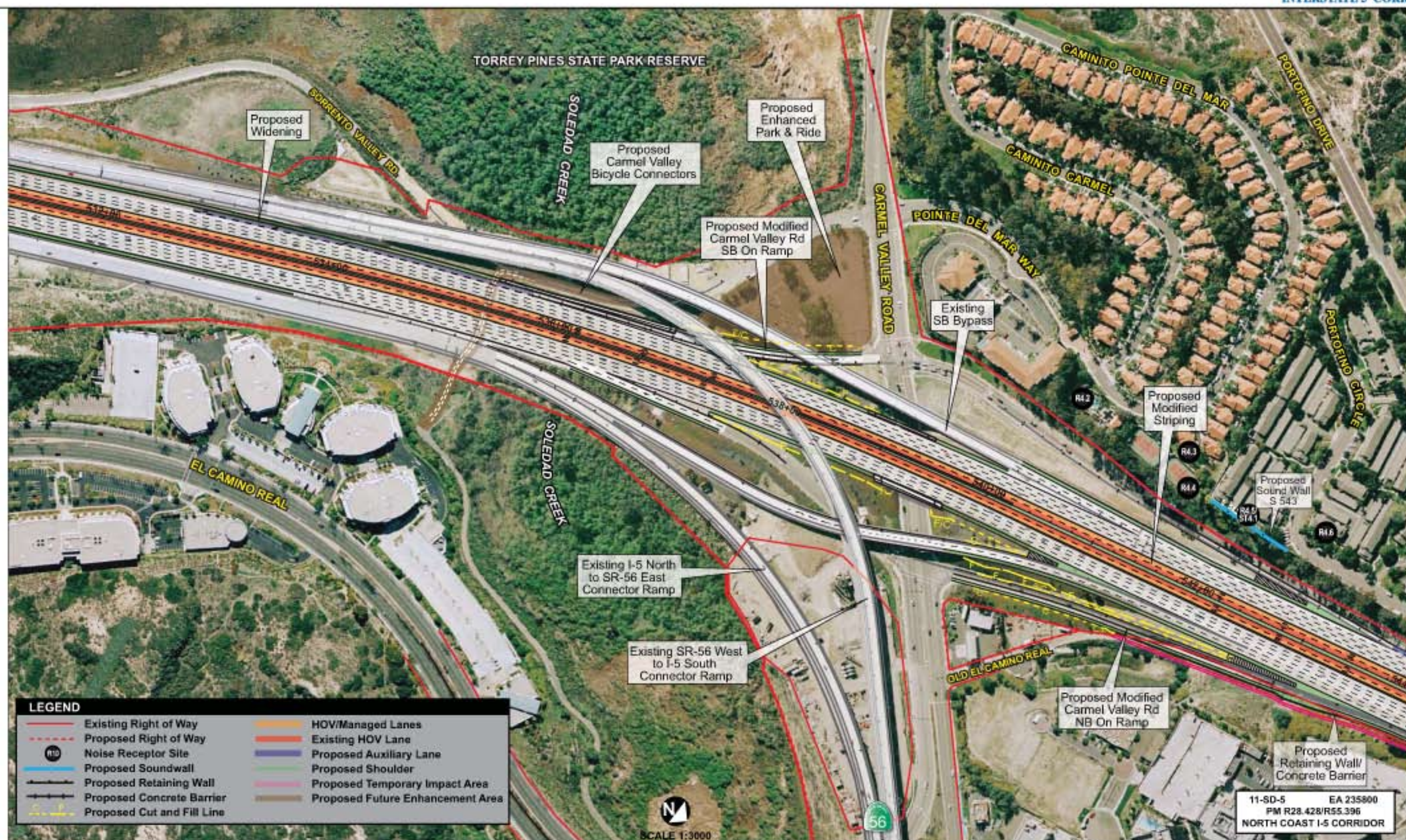
Figure 2-2.14h Project Features Map: 10+4 Buffer Alternative
