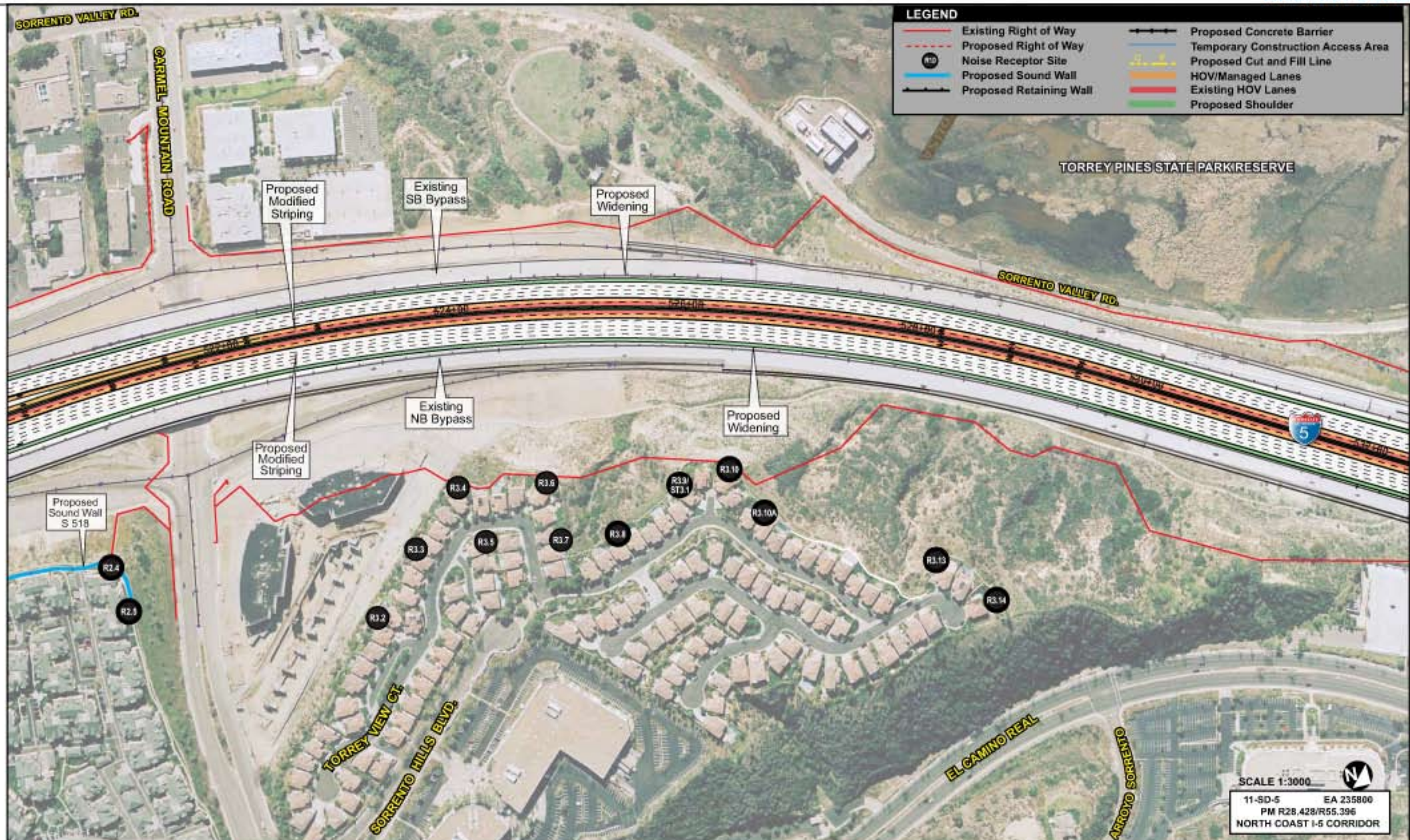
Figure 2-2.14g Project Features Map: 10+4 Buffer Alternative
