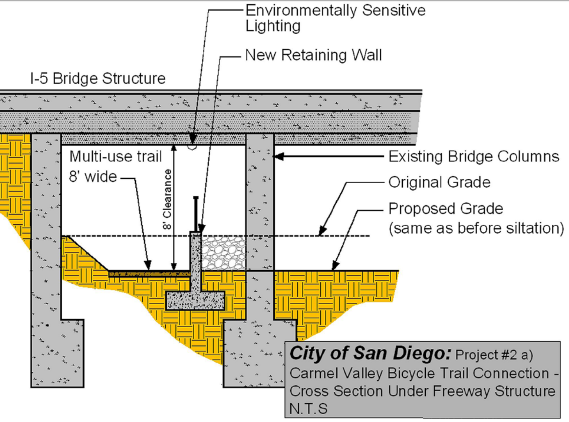
Proposed Pedestrian/Bike Trail Under I-5: Section/Elevation View Looking West
