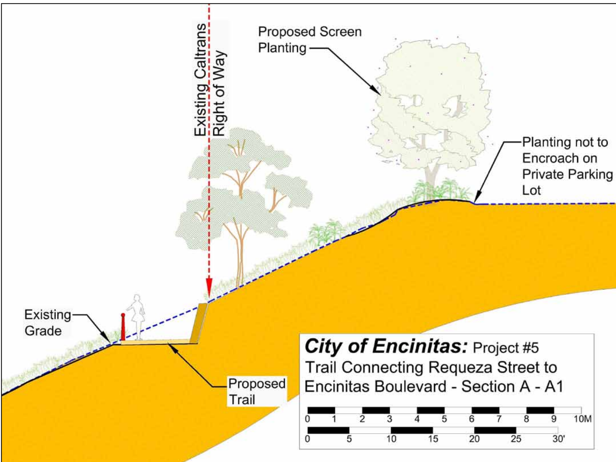
Proposed Pedestrian Trail Section/Elevation View Looking North
