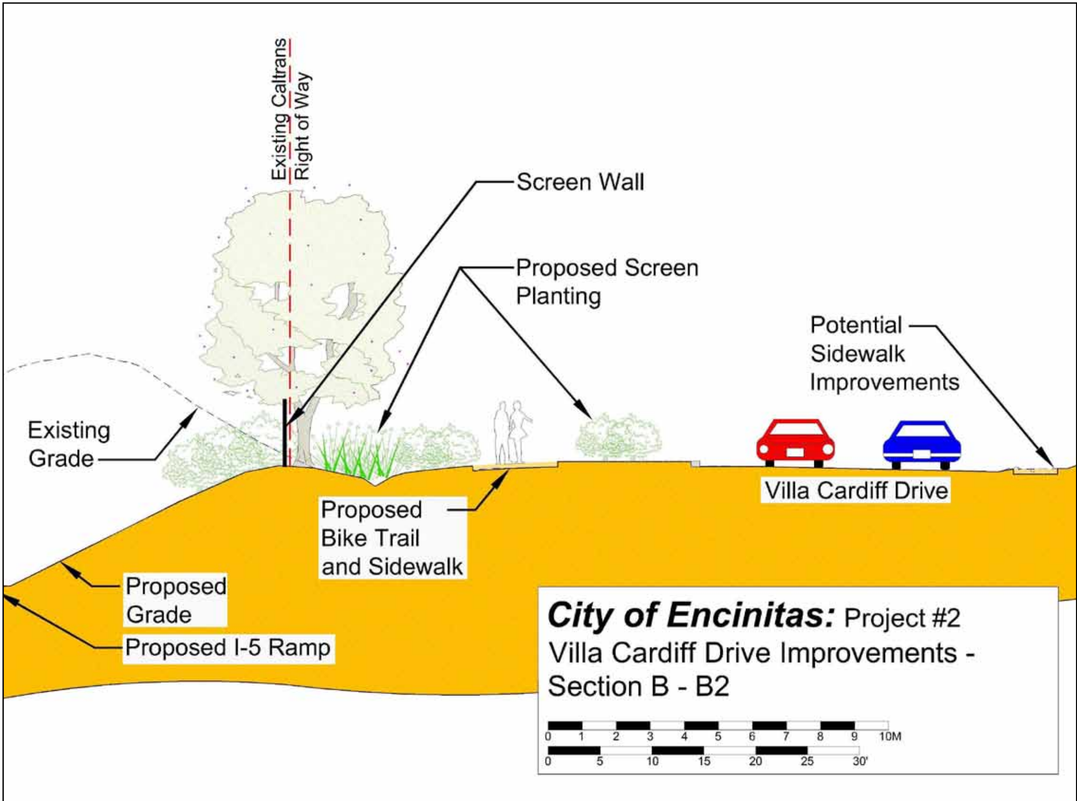
Proposed Pedestrian Trail & Re-vegetation Section/Elevation View Looking North
