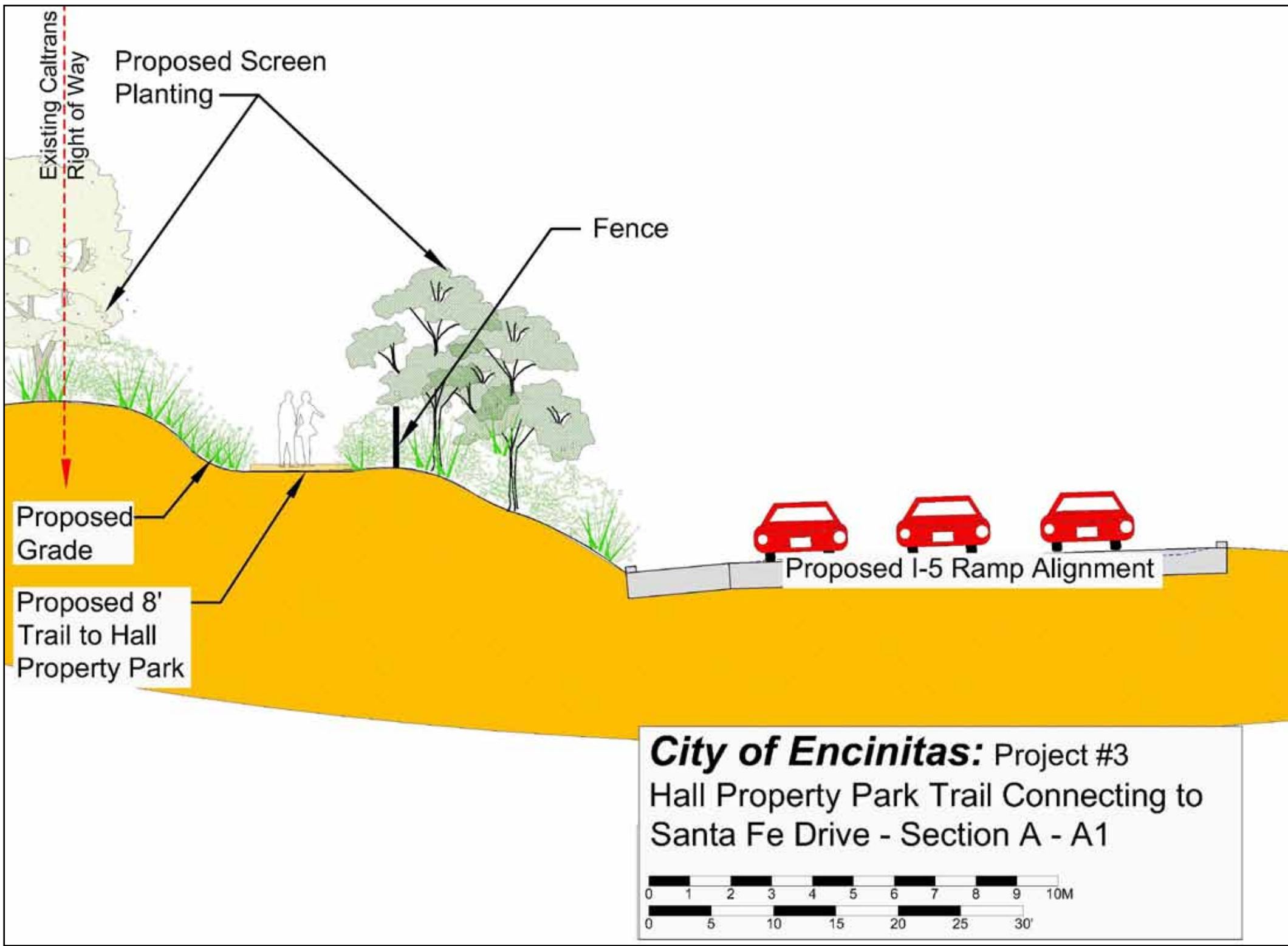
Proposed Pedestrian Trail Section/Elevation View Looking North
