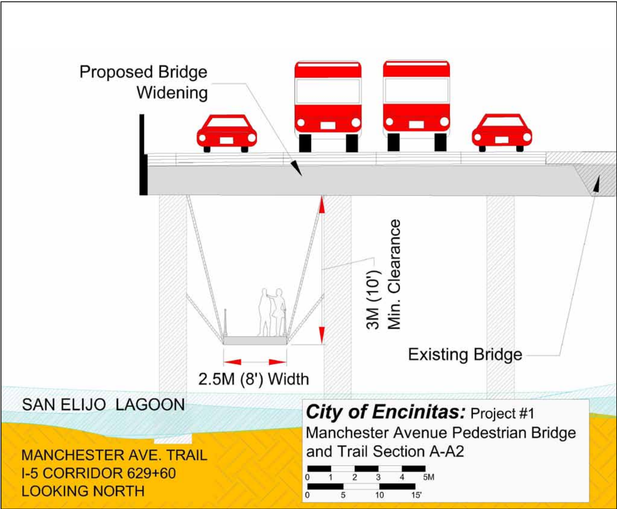
Proposed Suspended Pedestrian Bridge: Section/Elevation View Looking North
