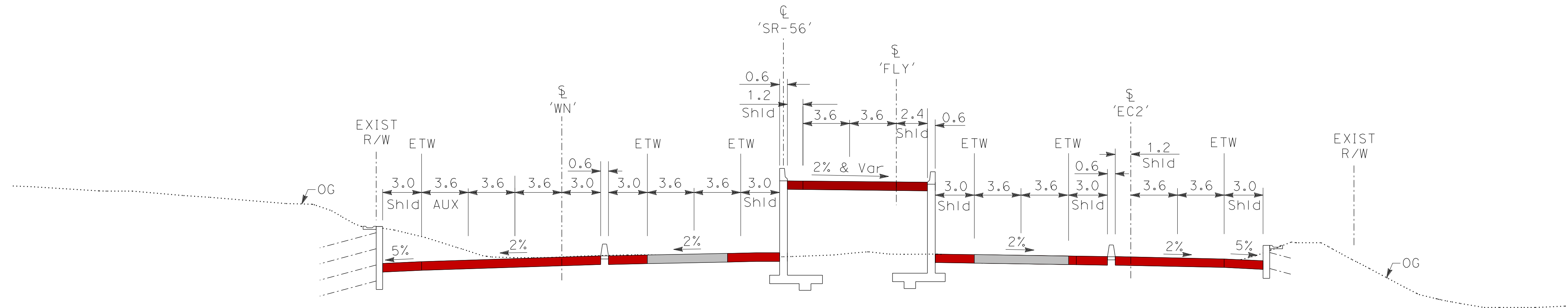
SECTION A-A I-5 / SR-56 INTERCHANGE
